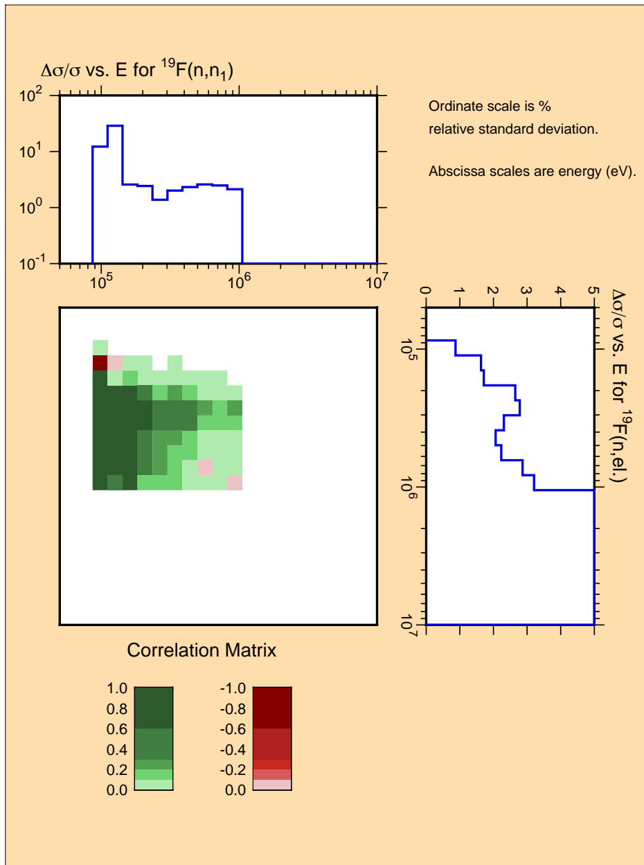
Figure 39: Covariance plot for the elastic and (n,n 1 ) reactions in the experimental evaluation for 19 F, demonstrating the channel-channel covariances possible when using the Reich-Moore-Limited resonance representation.
